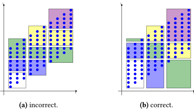
Figure 4. Seidel-2d algebraic tiling dependence violation. Tiles of same color should be executed concurrently.
