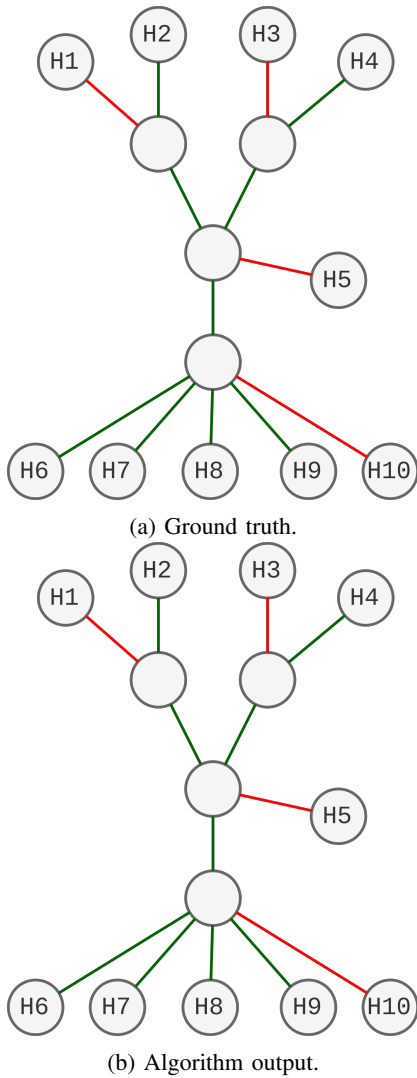
Fig. 7: Run 2. Perfect prediction: 100% precision and F_1 -score.
