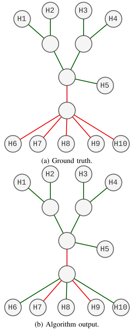
Fig. 8: Run 3. Erroneous prediction: 0% precision and 66.\bar{6}\% F_1 -score.
