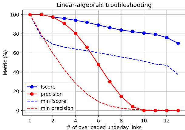
Fig. 4: Simulation results on all 8192 overloading cases. The continuous lines show the performance of linear-algebraic troubleshooting with Occam’s razor heuristic (Heuristic 1); and the dotted lines by relying only on lower and upper bounds (Heuristic 0).
