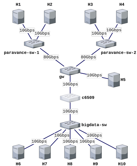
Fig. 2: Underlay infrastructure network.
