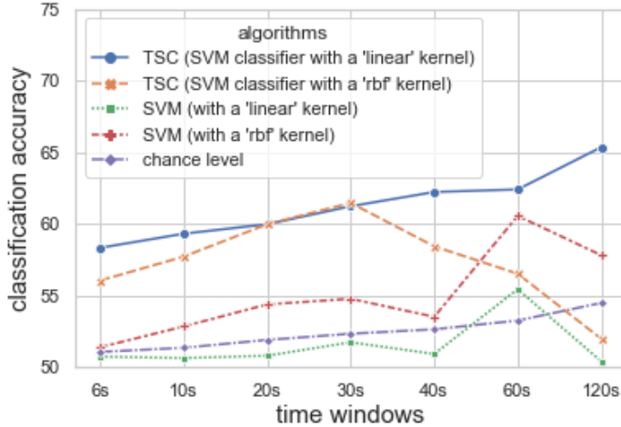
Fig. 3 Classification accuracy for each time window and algorithm, i.e., Euclidean SVM with both 'linear' and 'RBF' kernels and Riemannian TSC with an SVM classifier using both 'linear' and 'RBF' kernels.
