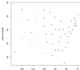
dist(state.x77) hclust("complete")
