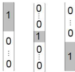
First three eigenvectors
