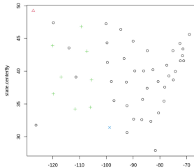
dist[state.x77] hclust ("ward.D2")
