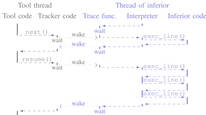
Fig. 5: The Python tracker runs the inferior in a thread.
