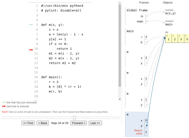
Fig. 10: A Python Tutor session from a EasyTracker trace.
