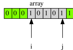
Fig. 1: A visualization tool built on top of EasyTracker to visually represent the concept of loop invariant. The next line to execute is highlighted in the source code and the loop invariant visualization exhibits the principle of the algorithm.
