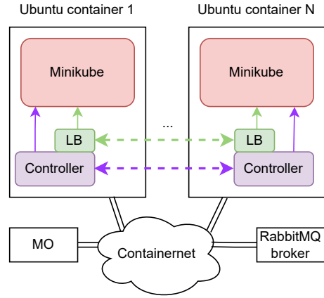
Figure 5. Testbed with containernet
