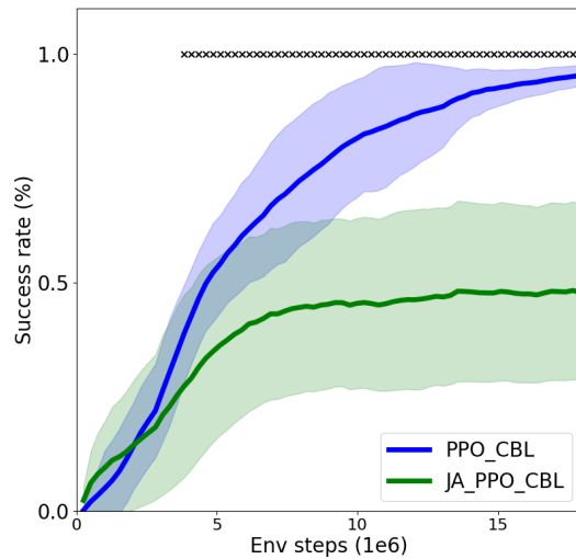
Figure 17. The joint attention experiment. The environments feature a test for recursiveness - infer if the peer knows that they are working together. The environments are same as the ones from figure 15(b), but with the addition of misleading cues - random cues given regardless of the agent (a random color). The peer gives misleading cues outside of joint attention (before the introductory sequence). The agent should ignore these cues, and use only cues given inside joint attention. The figure compares the success rate (mean +/- std over 8 seeds) of the agent trained on the environments with both regular and misleading cues ("JA_PPO_CBL"), to the agent trained on the environments with only regular cues ("PPO_CBL(train)" from figure 15(b)). The figure shows that the agent unable to master the Joint Attention variant.
