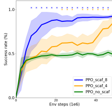
Figure 3. The scaffolding experiment. The comparison of agents trained on multiple environments of varying difficulty to that trained on an unscaffolded environment. The figure shows success rates on the testing environments (mean \pm std over 8 seeds) and the cross marks depict statistical significance ( p = 0.05 ) with respect to the "no_scaf" baseline. Only the scaffolded agents ("scaf_4" and "scaf_8") solve the environment, and the scaffolding with eight difficulty levels is more sample efficient.
