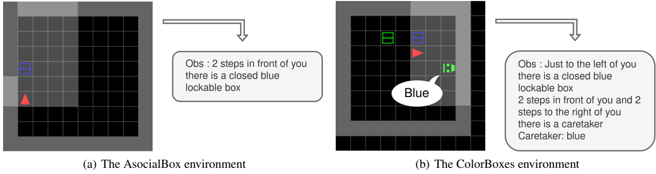
Figure 23. Two environments used in the experiments with large language models. The observations are parsed into pure text.
