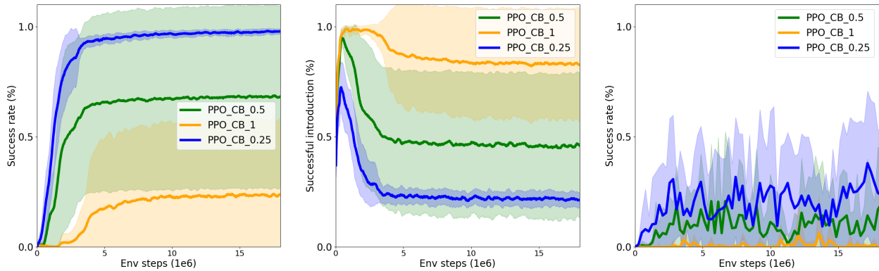
(a) Imitation experiments performance (success rate) on the training environments. (b) The percentage of successful introductory sequences on the training environments. (c) Imitation experiments performance (success rate) on the testing environment.
