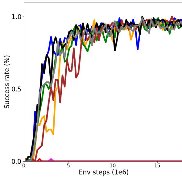
Figure 16. Per-seed performance on the training environments of the agent from figure 15(a) ("PPO_CBL(train)"). The figure shows that the agent is able to solve the training tasks efficiently, but that there are two unstable seeds which result in the success rate of 0%.
