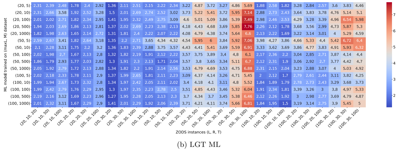
Fig. 20 Results for ML on ZODS instances for different training datasets, similar to Fig. 18, with L \in \{20, 50, 100\} , R \in \{10, 20, 30\} and |T| \in \{20, 50, 100\}
