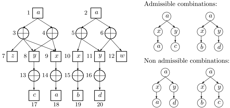
Figure 3: Left panel: An e-colored ad-AND/OR graph. Right panel: For \mathcal{O} = \{1, 2\} , there are four combinations between \mathbb{C}(G/C_1^2) and \mathbb{C}(G/C_2^2) ; only two of them are admissible.
