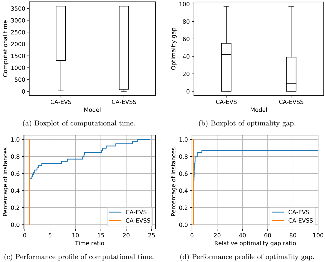
Figure 8: Performance profiles and boxplots comparing CA-EVS and CA-EVSS.
