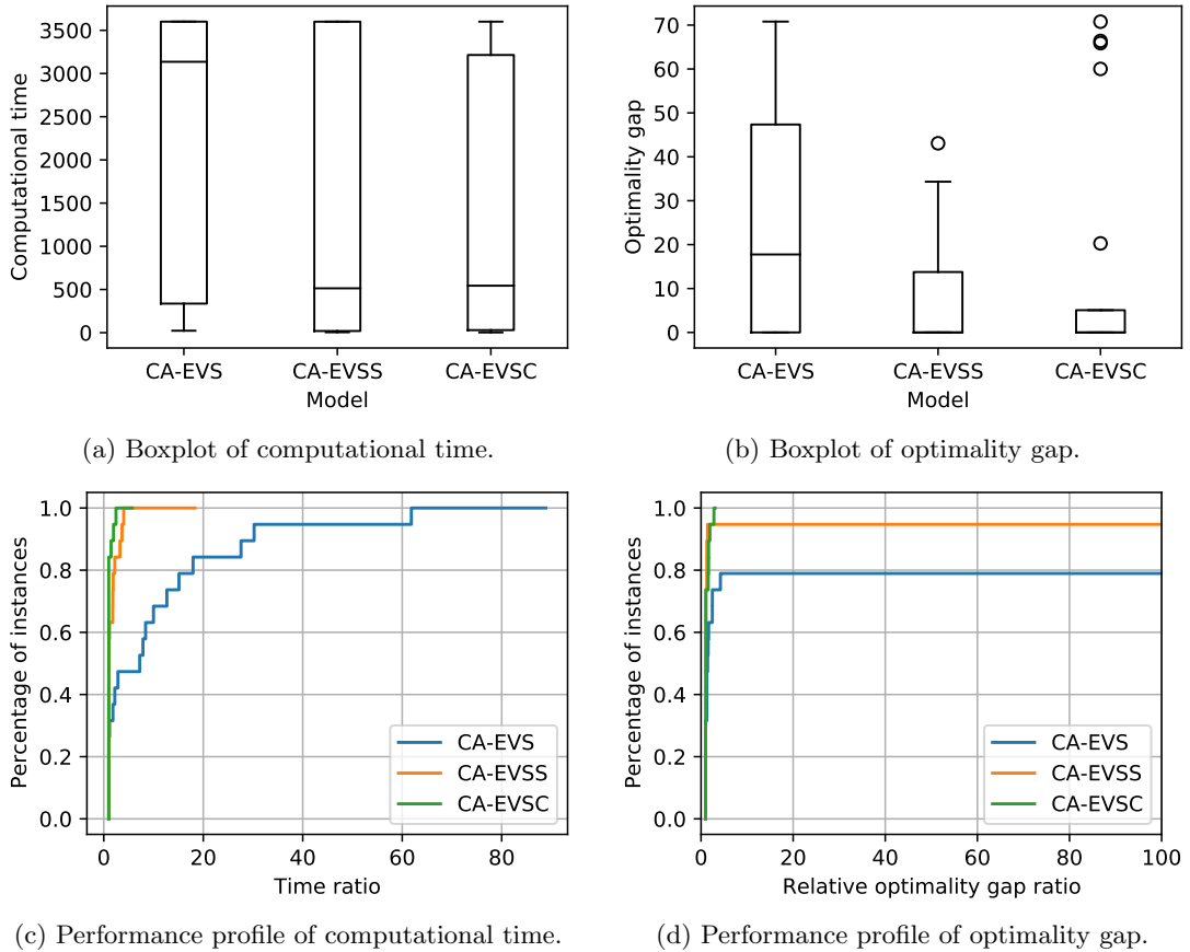
Figure 9: Performance profiles and boxplots comparing CA-EVS, CA-EVSS, and CA-EVSC when c is convex.
