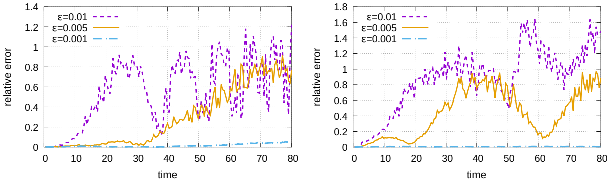
Figure 4: The relative error of the first-order model, for several values of \varepsilon , in long time. Left: The magnetic bottle case, Right: The asymmetric magnetic field case.
