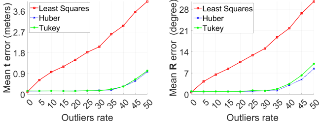
(a) Comparison with robust methods, translation error (m). (b) Comparison robust methods, rotation error (degrees).
