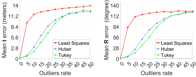
(a) Comparison with robust methods, translation error (m). (b) Comparison with robust methods, rotation error (degrees).
