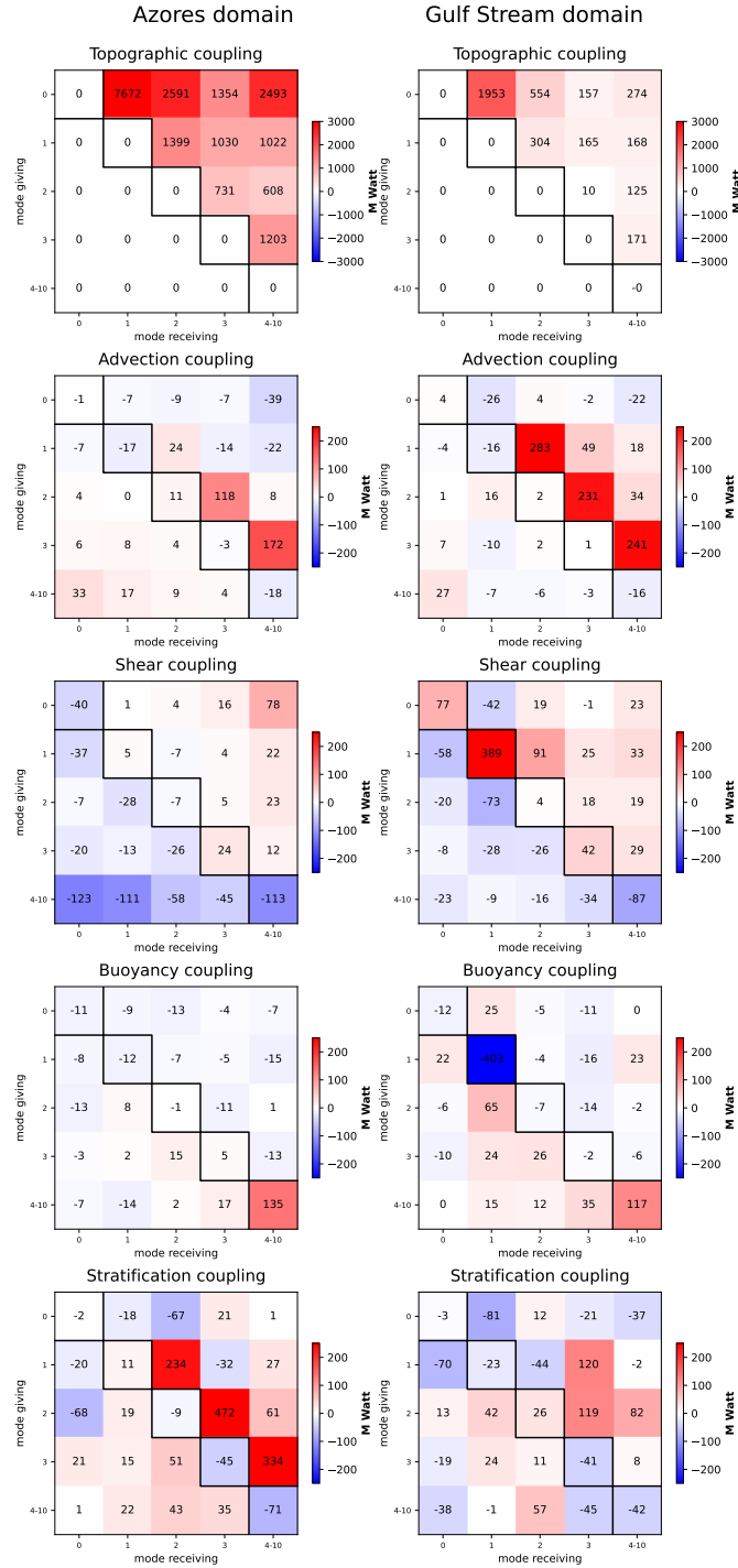
Fig. 2. Matrices K_{nm} summarising the mean energy transfer integrated over the whole subdomains between a mode n (row) and a mode m (column). The upper-right triangle is the anti-symmetric part, and the lower-left triangle (diagonal included) the symmetric part. The sign convention follows eq. (15): a positive value indicates a gain of energy for the reference –“receiving” – mode m from n mode and conversely. Modes 4 to 10 are grouped together. From top to bottom are the coupling caused by the topography, the internal tide advection by the background flow, the terms implying the horizontal and vertical shear of the background flow and the term implying the gradient of the buoyancy field (both variable and annual mean). Notice the different range of values in the colorbar for the topographic coupling terms compared to the other ones.
