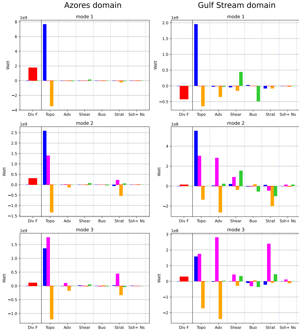
Fig. 3. Mean modal budget for modes 1 (top), 2 (middle row) and 3 (bottom) for the Azores domain (left) and the Gulf Stream (right) domains, as described by equation (15). The divergence of the modal flux is plotted in red, while others contributions are separated into the symmetric part (green) and the anti-symmetric part where interaction with lower modes and with higher modes (orange) are separated. The anti-symmetric part coming from low modes is furthermore separated into fluxes coming from the barotropic mode (blue) and fluxes coming from the baroclinic modes (fuchsia). A positive value means a gain of energy for the mode. Processes taken into account are Topo : C_{nm} , Adv : A_{nm} , shear : \nabla U_{nm} , ssh + Ns : S_{nm} , Buo : \nabla B_{nm} , Strat : N_{nm} .
