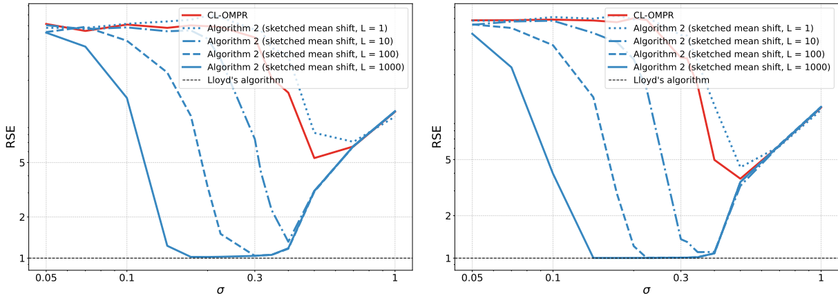
(b) Average RSE of CL-OMP for two sketch sizes (left: m = 200 ; right: m = 1000 ), and Algorithm 2 using sketched mean shift for L \in \{1, 10, 100, 1000\} .
