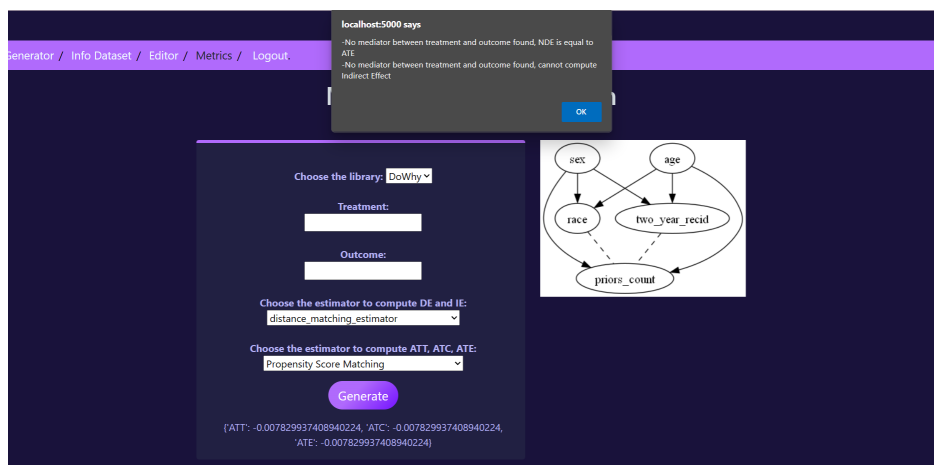
Figure 6: Measuring Discrimination Page
