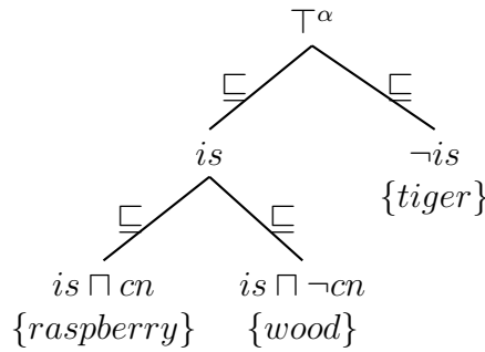
Figure 3: An example of an agents’ ontology after learning with the objects raspberry , then tiger , and then wood . cn stands for containsNutrients , iol for isOnLand , and is for isSmall .
