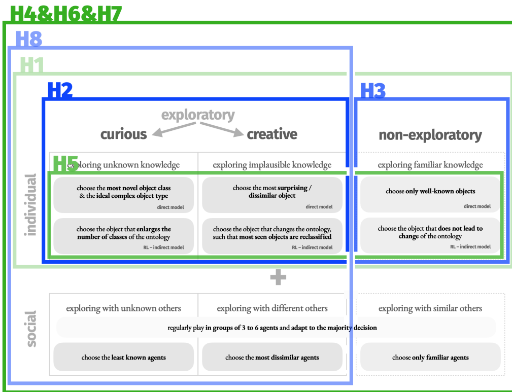
Figure 16: The hypotheses.
