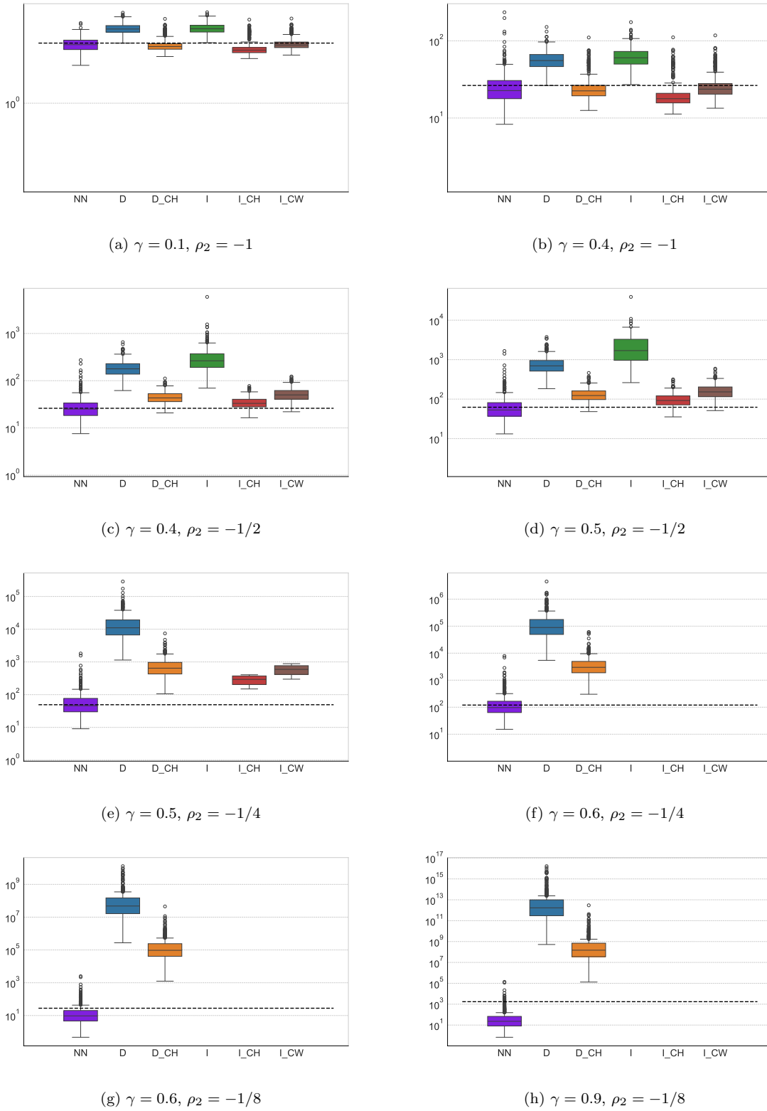
Figure 4: Boxplot (in a logarithmic scale) of the six estimators NN (purple), \widehat{\text{ES}}^{\text{D}} (blue), \widehat{\text{ES}}^{\text{D,CH}} (orange), \widehat{\text{ES}}^{\text{I}} (green), \widehat{\text{ES}}^{\text{I,CH}} (red) and \widehat{\text{ES}}^{\text{I,CW}} (brown) of the extreme ES at level 1 - \alpha_n = 1 - 1/(2n) on 500 replications of the Burr distribution. The real ES value is depicted by a horizontal black dashed line.
