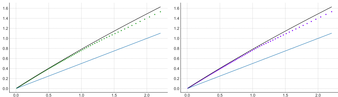
Figure 1: ES log-spacings associated with a Burr distribution ( \gamma = 1, \rho_2 = -1/2 ), see Table 1 for the parameterization. Black curve: theoretical function (x_1, g_1(x_1, \log(n/k))) ; blue line: first order approximation (x_1, \gamma x_1) with \varphi = 0 and \Psi_1(\cdot) = -\log(1 - \gamma) ; green dots (left panel): empirical pointwise estimation (\log(k/i), \hat{S}_{i,k}) ; purple dots (right panel): NN estimation (\log(k/i), \tilde{g}_{1,\hat{\theta}}^K(\log(k/i), \log(n/k))) with i \in \{1, \dots, k - 1\} , k = 100 and n = 500 .
