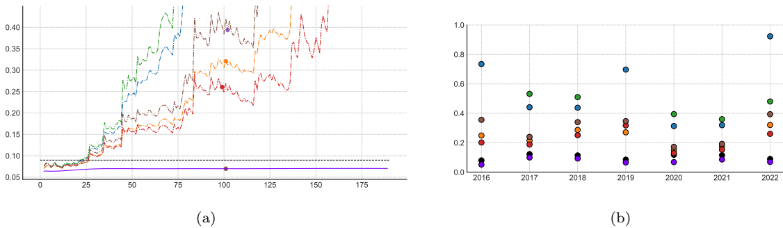
Figure 5: Illustration on real data: Estimation of the extreme ES associated with empirical (black), \widehat{ES}^D (blue), \widehat{ES}^{D,CH} (orange), \widehat{ES}^I (green), \widehat{ES}^{I,CH} (red), \widehat{ES}^{I,CW} (brown) and NN (purple) estimators. (a): Estimated ES as functions of k \in \{2, \dots, n - 1\} for the year 2022. The empirical estimate is depicted with a horizontal black dashed line. (b): Estimated ES at the selected anchor point for all considered years. The vertical axis is clipped between 0 and 1.
