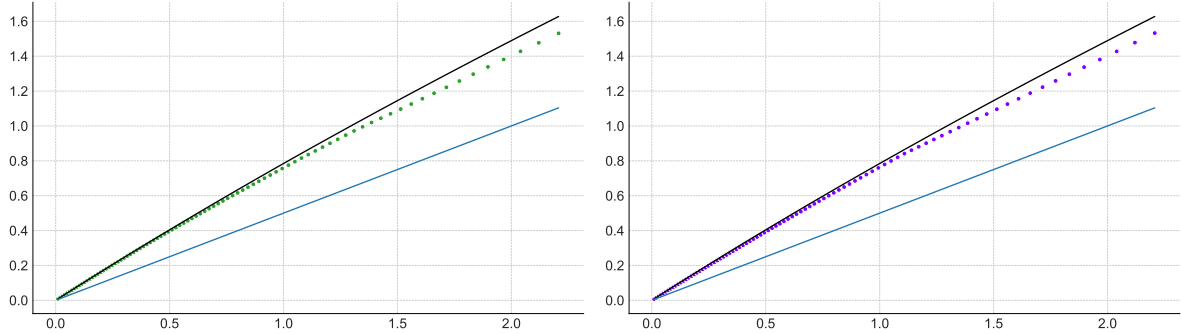
Figure 1: ES log-spacings associated with a Burr distribution ( \gamma = 1, \rho_2 = -1/2 ), see Table 1 for the parameterization. Black curve: theoretical function x_1 \mapsto g_1(x_1, \log(n/k)) ; blue line: first order approximation x_1 \mapsto \gamma x_1 with \varphi = 0 and \Psi_1(\cdot) = -\log(1 - \gamma) ; green dots (left panel): empirical pointwise estimation (\log(k/i), \hat{S}_{i,k}) ; purple dots (right panel): NN estimation \tilde{g}_{1,\hat{\theta}}^K(\log(k/i), \log(n/k)) with i \in \{1, \dots, k-1\} , k = 100 and n = 500 .
