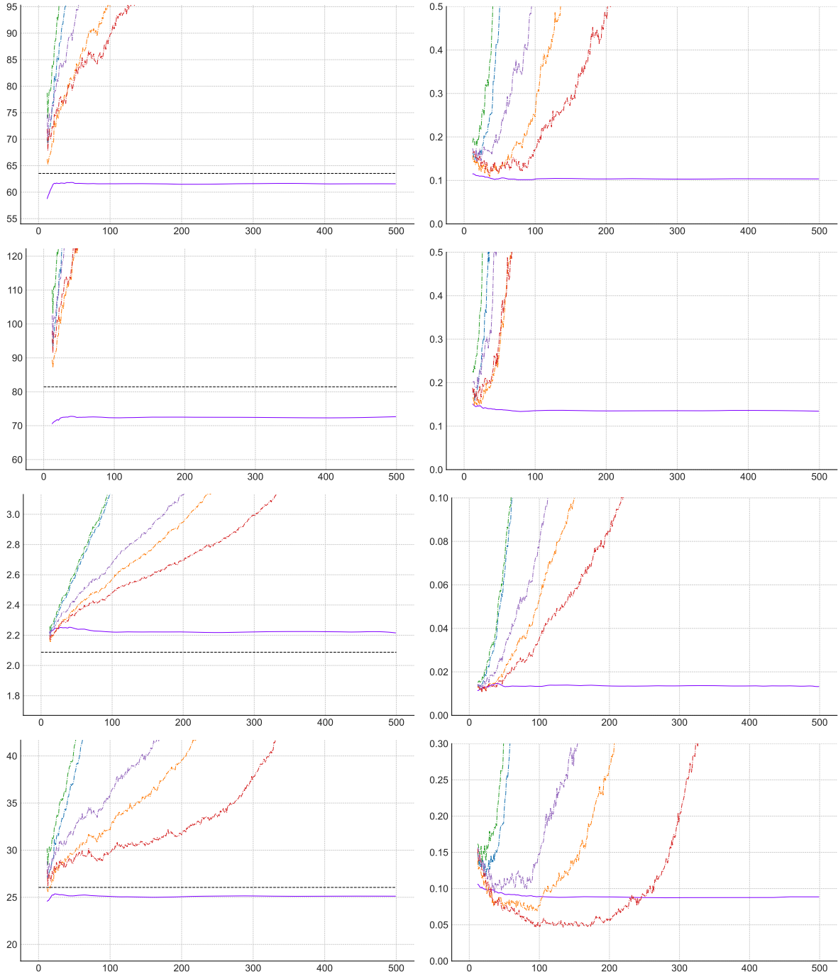
Figure 3: Illustration on simulated data sets of size n = 500 from GPD, Fisher-Snedecor (both with \gamma = 0.4 ) and Burr distributions with (\gamma = 0.1, \rho = -1/4) and (\gamma = 0.4, \rho = -1/2) from top to bottom. Median of the estimators (left panel) of the out-of-sample ES (black dashed line) at level 1 - \alpha_n = 1 - 1/(2n) and RMedSE (right panel), as functions of k \in \{2, \dots, n - 1\} , computed on R = 500 replications, associated with \widehat{\text{ES}}^{\text{D}} (blue), \widehat{\text{ES}}^{\text{D,CH}} (orange), \widehat{\text{ES}}^{\text{I}} (green), \widehat{\text{ES}}^{\text{I,CH}} (red), \widehat{\text{ES}}^{\text{I,CW}} (mauve) and NN (purple) estimators.
