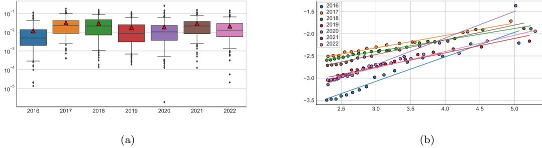
Figure 4: Illustration on real data. (a): Boxplot of the dataset (in a logarithmic scale) for each considered year. The mean is represented by a red triangle and the whiskers represent the 5th and 95th percentile. (b): Log quantile-quantile plots \log((n^{(j)} + 1)/i) \mapsto \log X_{n^{(j)} - i + 1, n^{(j)}}^{(j)} , for i \in \{1, \dots, \lceil (1 - \xi)n^{(j)} \rceil\} on the selected years j \in \{1, \dots, 7\} at probability level \xi = 0.90 .
