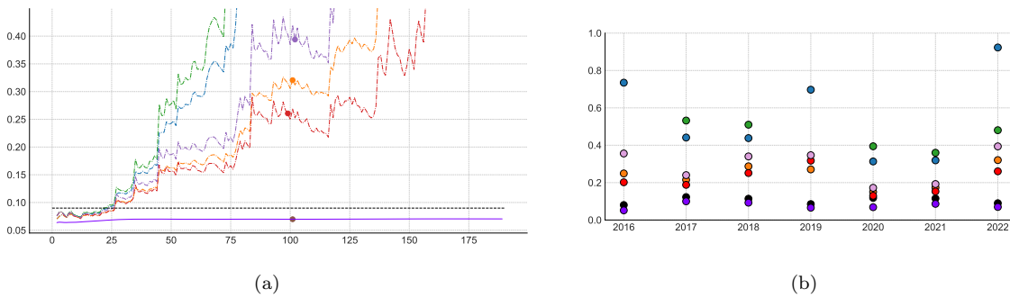
Figure 5: Illustration on real data: Estimation of the out-of-sample ES associated with empirical (black), \widehat{ES}^D (blue), \widehat{ES}^{D,CH} (orange), \widehat{ES}^I (green), \widehat{ES}^{I,CH} (red), \widehat{ES}^{I,CW} (mauve) and NN (purple) estimators. (a): Estimated ES as functions of k \in \{2, \dots, n-1\} for the year 2022. The empirical estimate is depicted with a horizontal black dashed line. (b): Estimated ES at the selected anchor point for all considered years. The vertical axis is clipped between 0 and 1.
