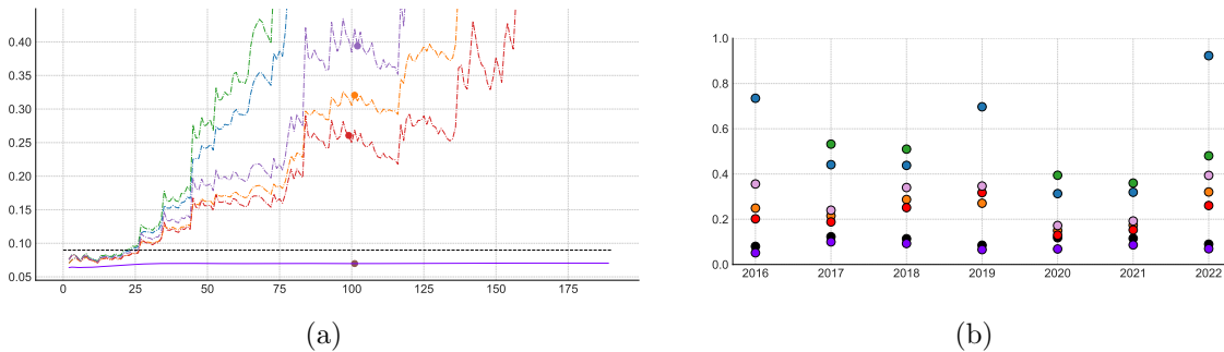
Figure 5: Illustration on real data: Estimation of the out-of-sample ES associated with empirical (black), \widehat{ES}^D (blue), \widehat{ES}^{D,CH} (orange), \widehat{ES}^I (green), \widehat{ES}^{I,CH} (red), \widehat{ES}^{I,CW} (mauve) and NN (purple) estimators. (a): Estimated ES as functions of k \in \{2, \dots, n - 1\} for the year 2022. The empirical estimate is depicted with a horizontal black dashed line. (b): Estimated ES at the selected anchor point for all considered years. The vertical axis is clipped between 0 and 1.
