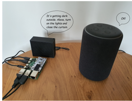
Fig. 1. IntraVox is composed of a Raspberry Pi 4B, sensors, speaker, Amazon Alexa and/or Google Home controlling smart home appliances.
