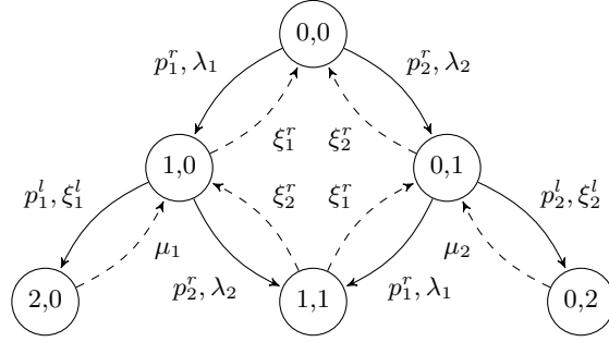
Fig. 1: RMLTSI DP_2 – the overall behavior of two dining philosophers
