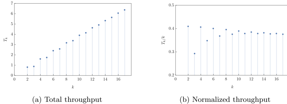
Fig. 3: Numerical evaluation of the throughput of DP_k for \lambda = 3 , \mu = 1 , \xi = 20
