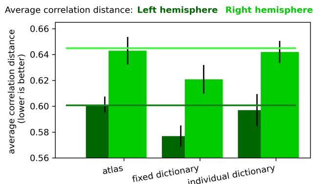
Figure 8: Quantitative comparison of the atlas fit at the whole-brain level. The quality metric obtained for three spatial models at the whole brain scale, across twenty validation folds. The three spatial models are the MMP1.0 atlas, a fixed dictionary and a subject-specific dictionary; \Delta_{atlas} , \Delta_{fixed} and \Delta_{individual} are displayed with bars representing between-fold variations. The horizontal lines represent the predictive accuracy of a voxel level model as defined in Eq. 6.
