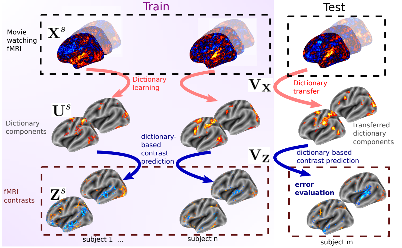
Figure 1: Representation of the individualized parcellation benchmark done in this work. ( left ) Dictionary learning is performed on naturalistic fMRI (mostly movie watching, see Table 1), resulting into individual-specific spatial components. From these components, one can learn to predict fMRI contrasts, using a regression approach. ( right ) Then, we transfer the dictionary onto new participants, obtaining a subject-specific dictionary, based on which we can then predict the amount of activation for the task fMRI contrasts observed in the training set. This is used to compute a prediction error that quantifies the overall goodness of fit of the model.
