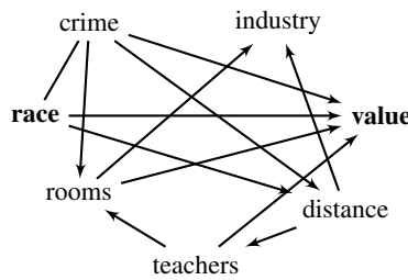
Figure 28: The graph for the Boston housing data set. 'Crime' is a possible confounder between 'race' and 'value'. The graph is produced using GES algorithm.
