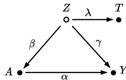
Figure 12: Simple measurement bias structure with linear coefficients.
