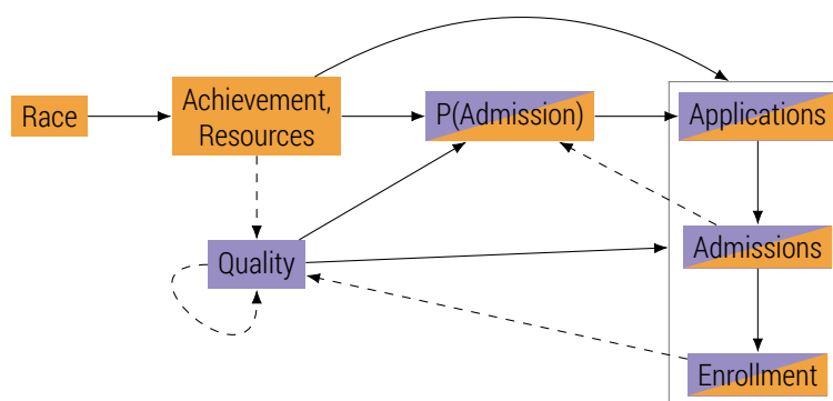
Figure 1. Simplified causal model of [1] with most of the variables being abstracted away. Students’ variables are orange, colleges’ variables are purple, while final variables defined for pairs of student and college have both colors. Dashed arrows represent dependency over past iterations.
