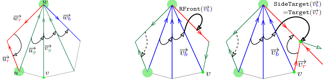
Figure 3: SCARST-OS. Left: green navigation. Right: blue navigation
