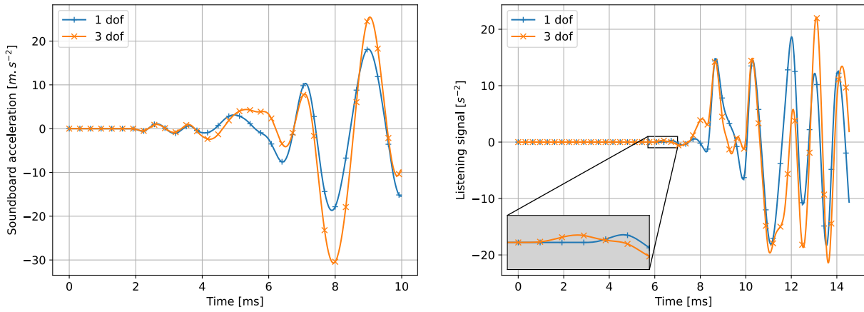
Figure 18: Soundboard acceleration at P_1 (left). Listening signal (right).
