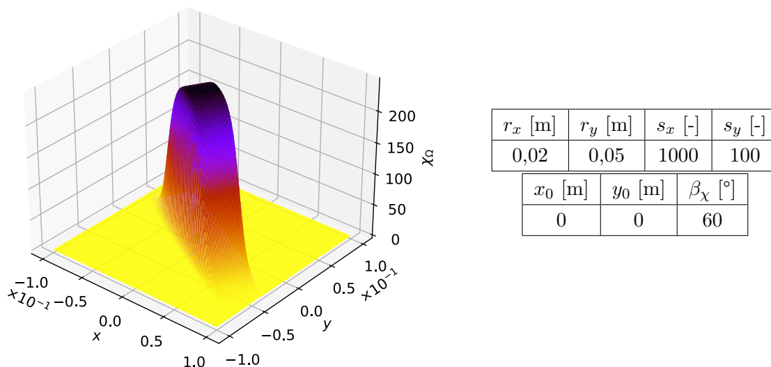
Figure 3: Distribution function \chi_\Omega .
