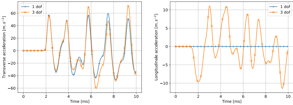
Figure 17: Acceleration of the end of the string for \alpha = 0 . Transverse (left), longitudinal (right).
