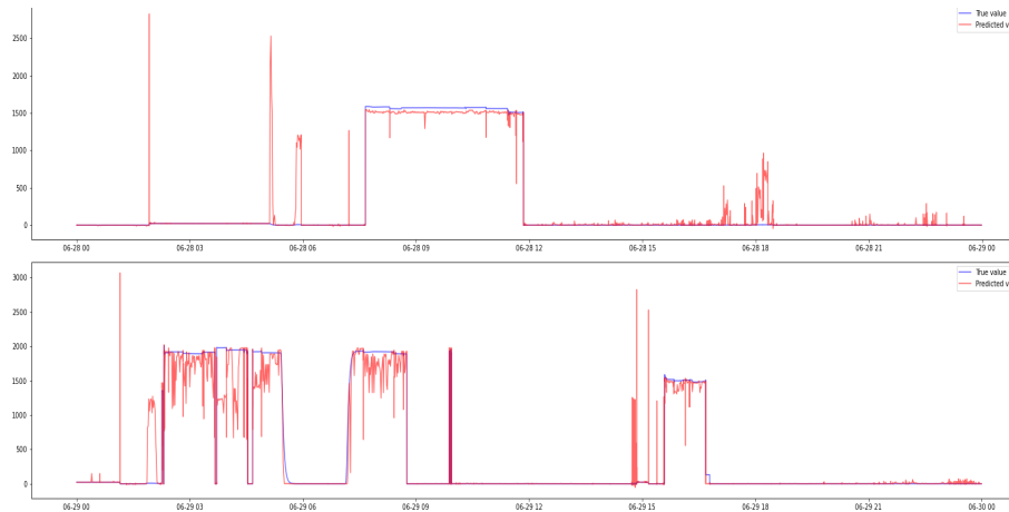
Fig. 5. Real vs Predicted consumption of Random Forest for the oven.
