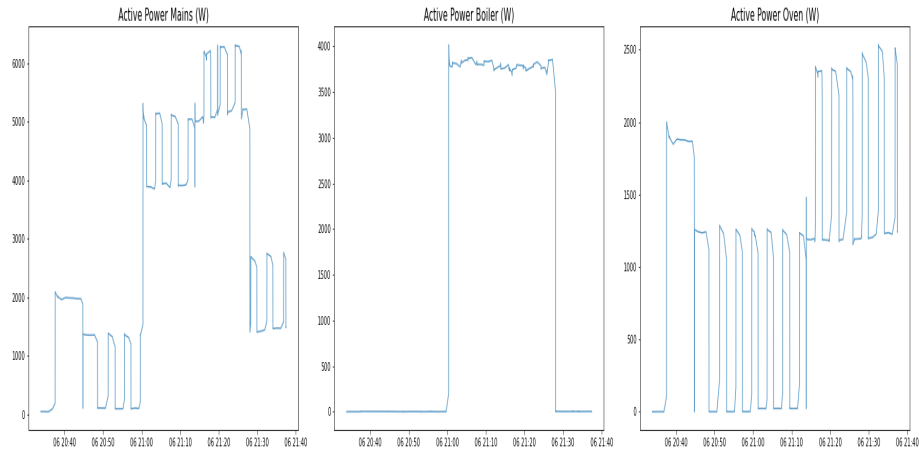
Fig. 2. Energy Consumption of appliances from 06/06/21 20:40 to 06/06/21 21:40
