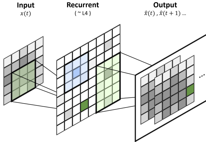
Fig 3: NILRNN self-supervised feature learning system architecture with partially-connected input and output. The green cells represent input and output feedforward connections. The blue cells represent local recurrent connections.
