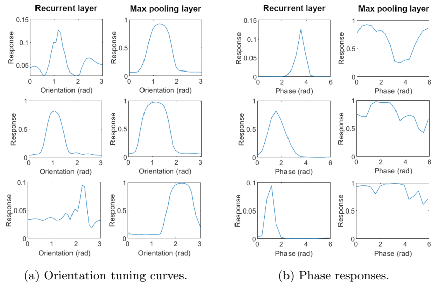
Fig. 7: Orientation tuning curves and phase responses of three representative neurons of each layer of an NILRNN trained with shifting images as input. The positions of the three neurons in both layers are (28,10) (top), (23,38) (middle) and (21,13) (bottom).
