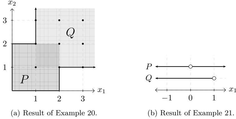
Figure 1: Visual representation of the models resulting from Examples 20 and 21.
