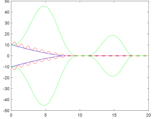
Figure 2. An illustration for Corollary 2
