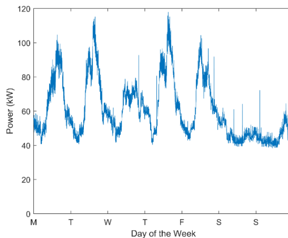
Fig. 3 – DEEC building's load diagram.
