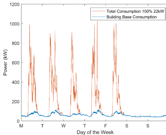
Fig.7 – Building’s load diagram with 100% EV penetration and 22kW
