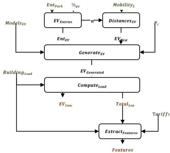
Fig 1 - Block diagram of the impact assessment methodology. Inputs are highlighted in green, outputs in red.
