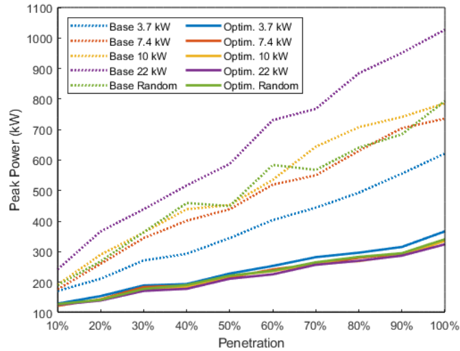
Fig. 9 - Comparison of the peak power in scenarios with and without charging management with 12 hours of user stay time.
