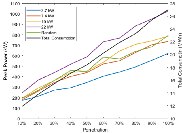
Fig.6 - Peak power and total energy consumption for different charging powers and EV penetration levels.
