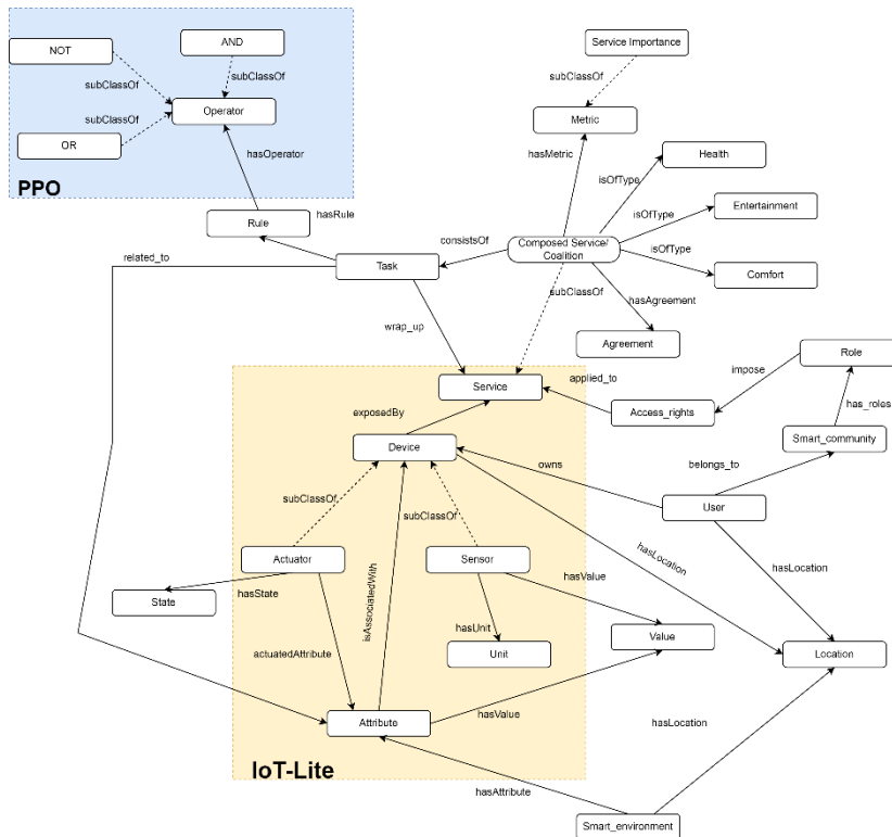
Fig. 2. Excerpt of a Collaborative CPS Service Ontology
