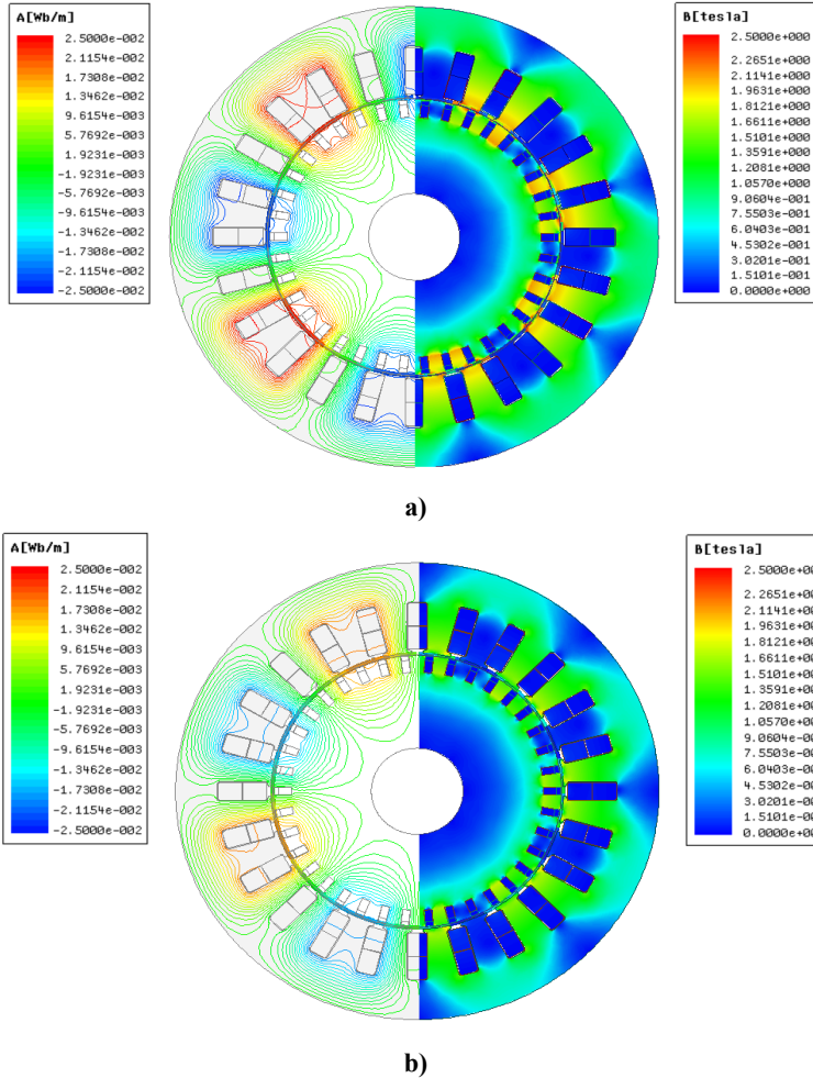
Fig.7. Magnetic flux lines and magnetic flux density distribution a) initial machine b) proposed machine.
