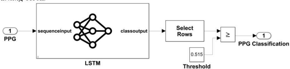
Fig. 3. Deep Learning block, with a PPG input, LSTM model and PPG classification.
