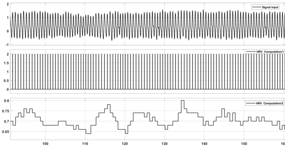
Fig. 7. Display output of the Simulink ® system of a PPG signal of 160 seconds. The PPG input signal, peak detection and HRV estimation are represented in the first, second and third plot, respectively.
