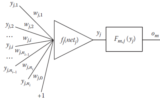
Figure 2. Connection of a neuron j with the rest of the network (extracted from [38])
