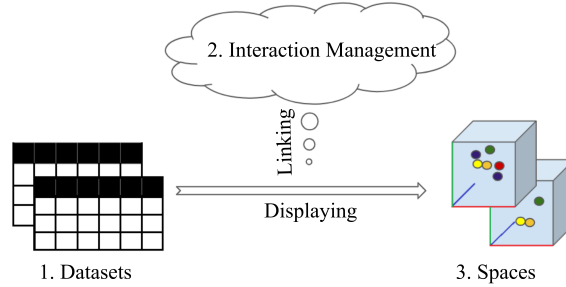
Fig. 1. Overview of the Spaces approach: reading from the datasets (1); a visualization instance is added to the interaction manager (2) for coordination techniques (Brushing and Navigational Slaving); data is rendered in the virtual environment, in the Spaces graphical representation (3).
