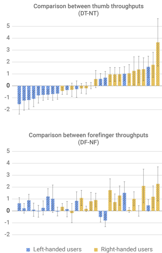
Fig. 9. Comparison of (dominant to non-dominant) thumb throughputs and forefinger throughputs for corresponding participants, where yellow (dotted) indicates right-handed and blue (lined) indicates left-handed users with error bars denoting \pm 1SD . The results have been arranged in an increasing order as per DT-NT.
