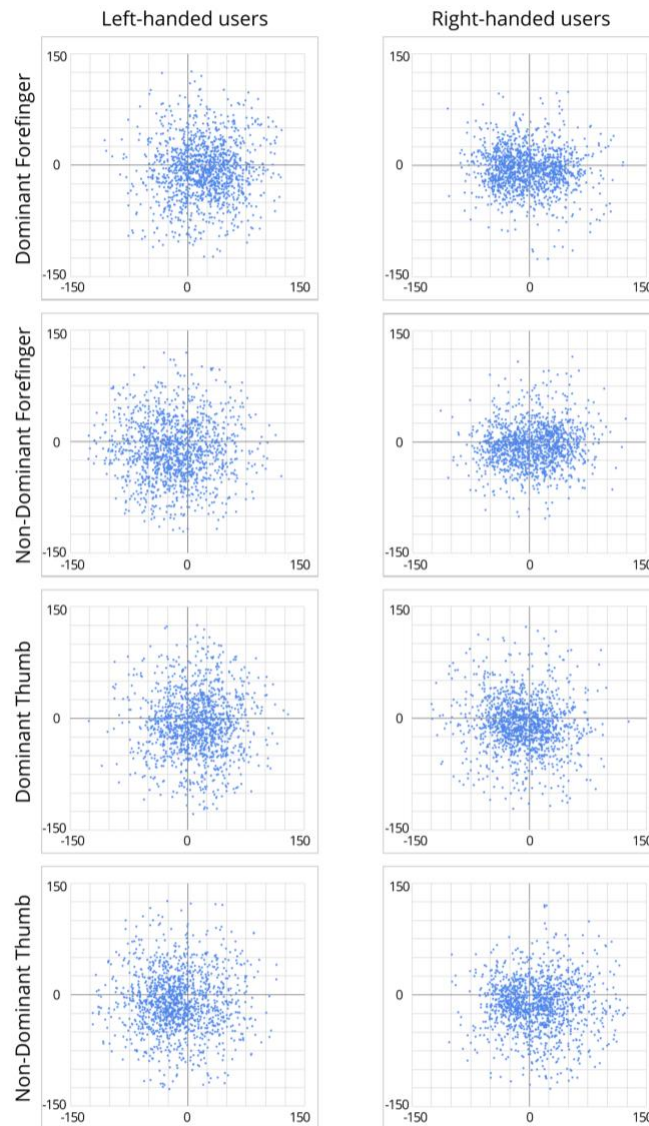
Fig. 10. Scatter plots of touches for different combinations
