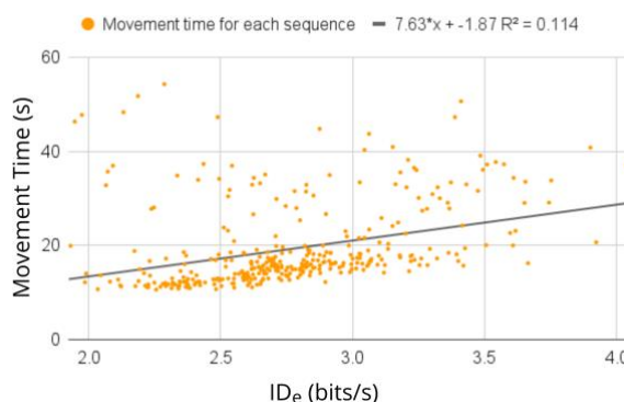
Fig. 8. Plotting movement time v/s index of difficulty for each sequence
