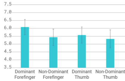
Fig. 6. Overall comparison between throughputs (error bars for 95% CI)
