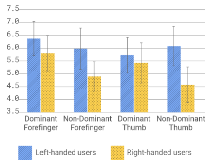
Fig. 7. Comparing throughputs across left and right-handed individuals (error bars for 95% CI)
