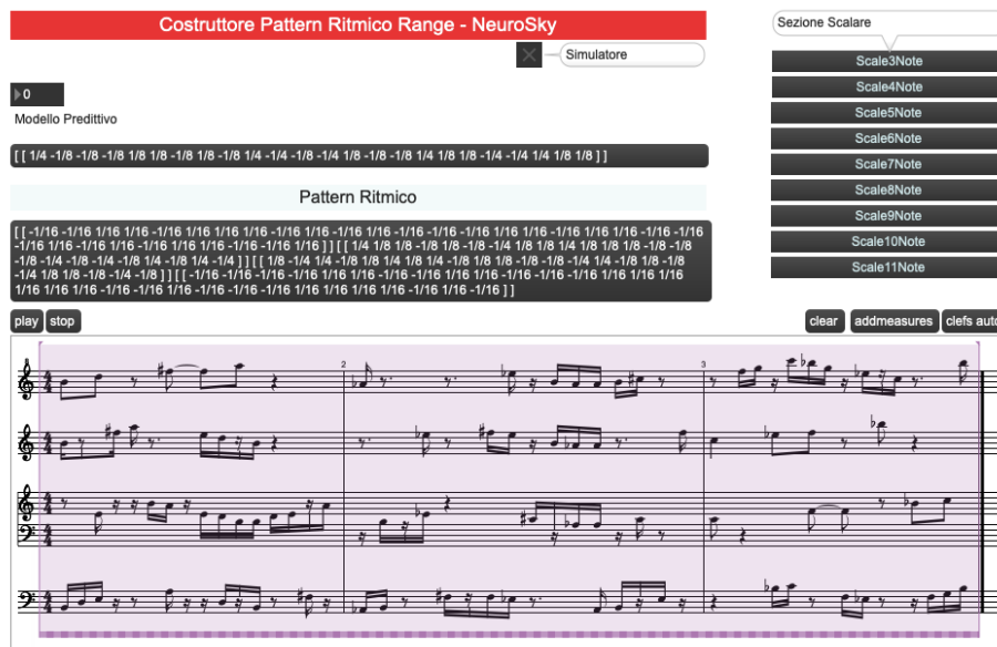
Fig. 5. User interface of the Polyphony Generator module.
