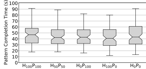
Fig. 5: Boxplots of pattern completion times for the different techniques.
