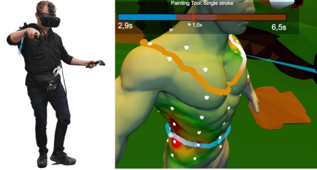
Fig. 12. VRTactileDraw driving a 52-actuator tactile vest mockup, and the users' view inside an HTC Vive
