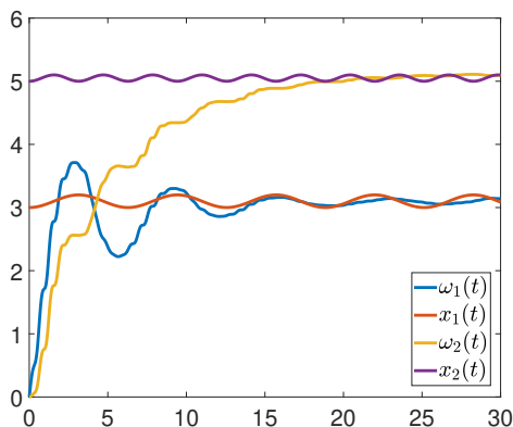
Fig. 2. Example 2. Nonlinear regression for a system given in a form (36).
