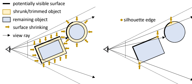
Fig. 2. (left) Geometric occluder shrinking needs to erode the entire object geometry to determine disocclusions, which is difficult to do analytically in 3D. (right) It is sufficient to only chisel away areas at the silhouette edges, which we call trim regions . This can be done using screen-space rasterization.
