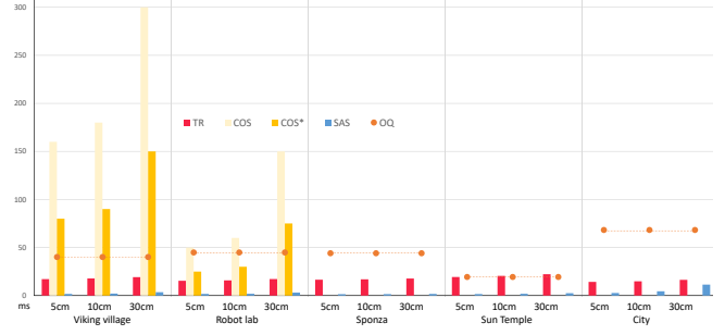
Fig. 14. Runtime comparison for various methods, scenes and viewcell sizes |\Delta| , reported in ms. “COS*” (yellow) is the time of “COS” (light yellow) scaled by 0.5\times to estimate runtime on the modern RTX 4090 GPU used in our experiments (data only available for Viking village and Robot lab). “OQ” (orange line) gives the runtime of the from-viewpoint OQ method, which has to recompute a new PVS for every frame.
