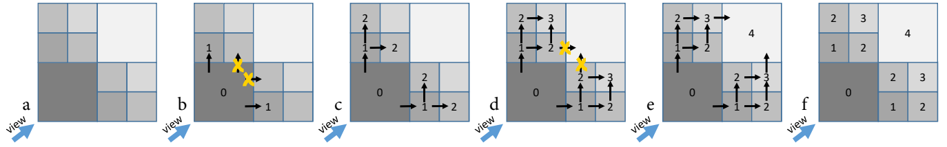
Fig. 10. An example of more complex traversal in the octree. (a) We select the start node based on the view direction. (b) From the start node, we move horizontally and vertically. We need to determine the appropriate neighbor nodes that would block other direct neighbors and process those first. (c) We proceed with traversal, until we arrive at another ambiguous location. (d) We need to ensure not to enter nodes prematurely, i.e. nodes that must wait for additional dependencies to be processed first. (e) All required neighbors have been processed. (f) We can move on and arrive at a final layer ordering.
