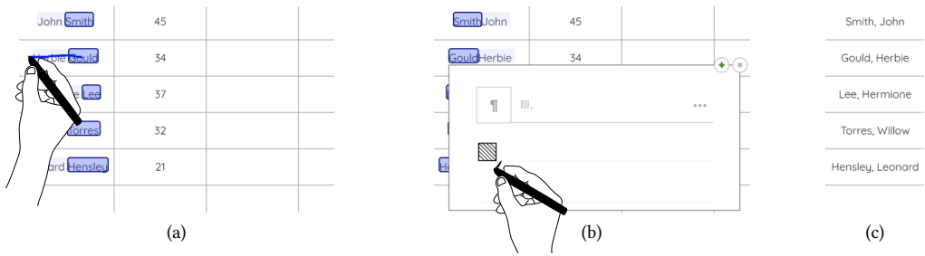
Fig. 18. Inverting first name and surname (John Smith \rightarrow Smith, John) by direct value-level manipulation as in Figure 11, but for all cells at once: (a) dragging the generalized surname subcell selection to the left; (b-c) inserting a comma followed by a white space between all surnames and first names.
