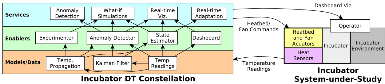
Figure 1: A conceptual representation of the incubator system and its digital twin.
