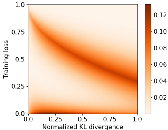
(a) The difference between the binary KL bound on the population loss and the one obtained via sub-Gaussianity for a bounded loss function.
