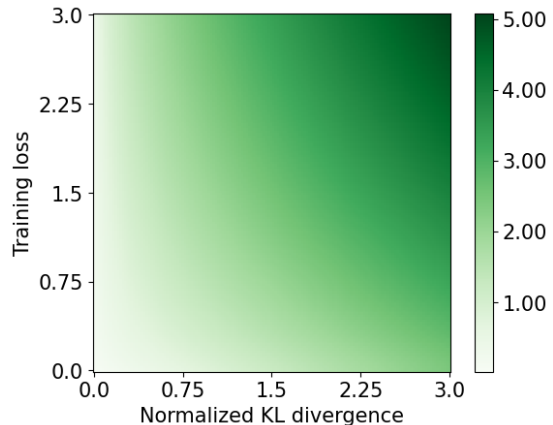
(b) The difference between the sub-Poissonian bound on the population loss obtained via (48) and the one obtained via (45).
