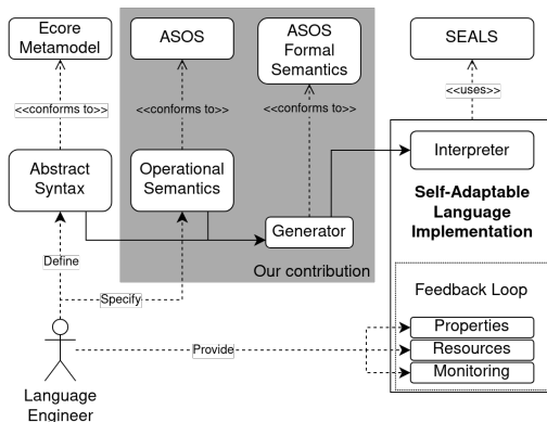
Figure 1. Approach overview
