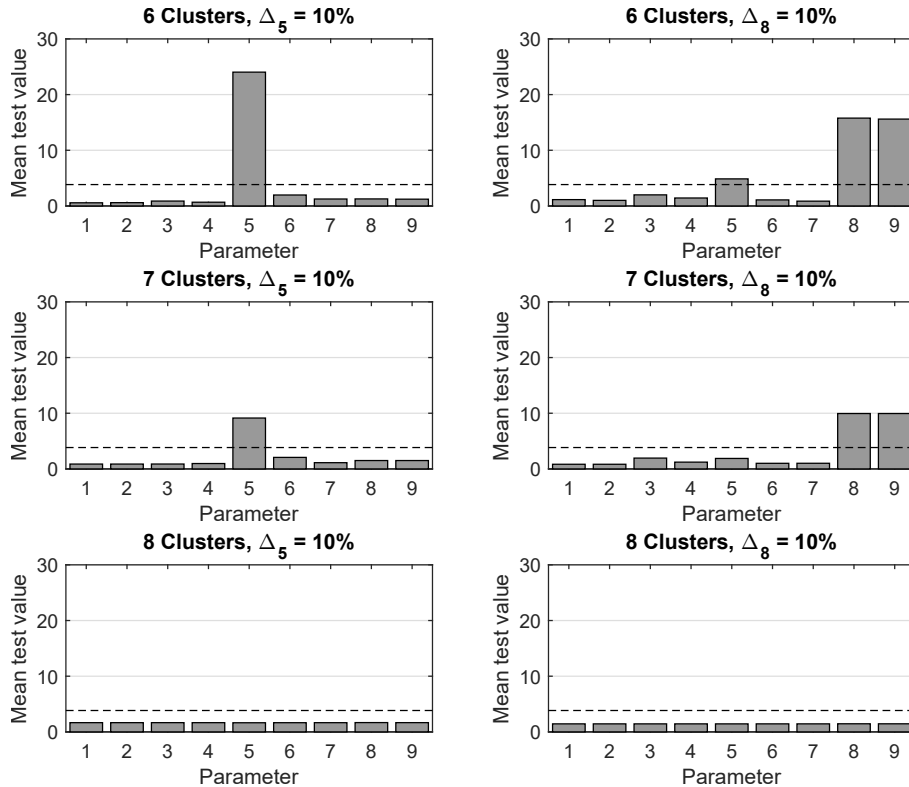
Figure 12: Mean test shift due to changes in parameter 5 and 8 for a cluster with 6 clusters (top), seven clusters (center), and eight clusters (bottom)
