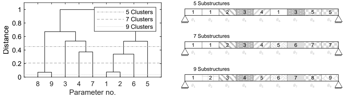
Figure 7: Cluster tree for pin-supported beam (left) with corresponding substructure arrangement for five, seven, and nine substructures (right)
