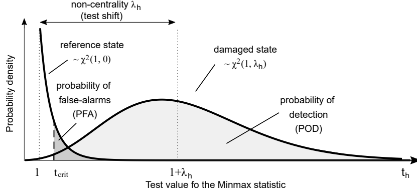
Figure 1: Statistical distribution of the minmax test statistic from Eq. (12)
