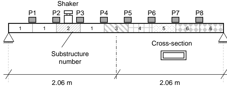
Figure 10: Optimal substructure arrangement with six parameter clusters
