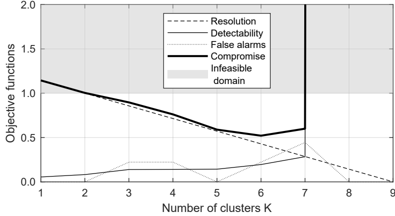
Figure 9: Objective functions for a varying number of clusters
