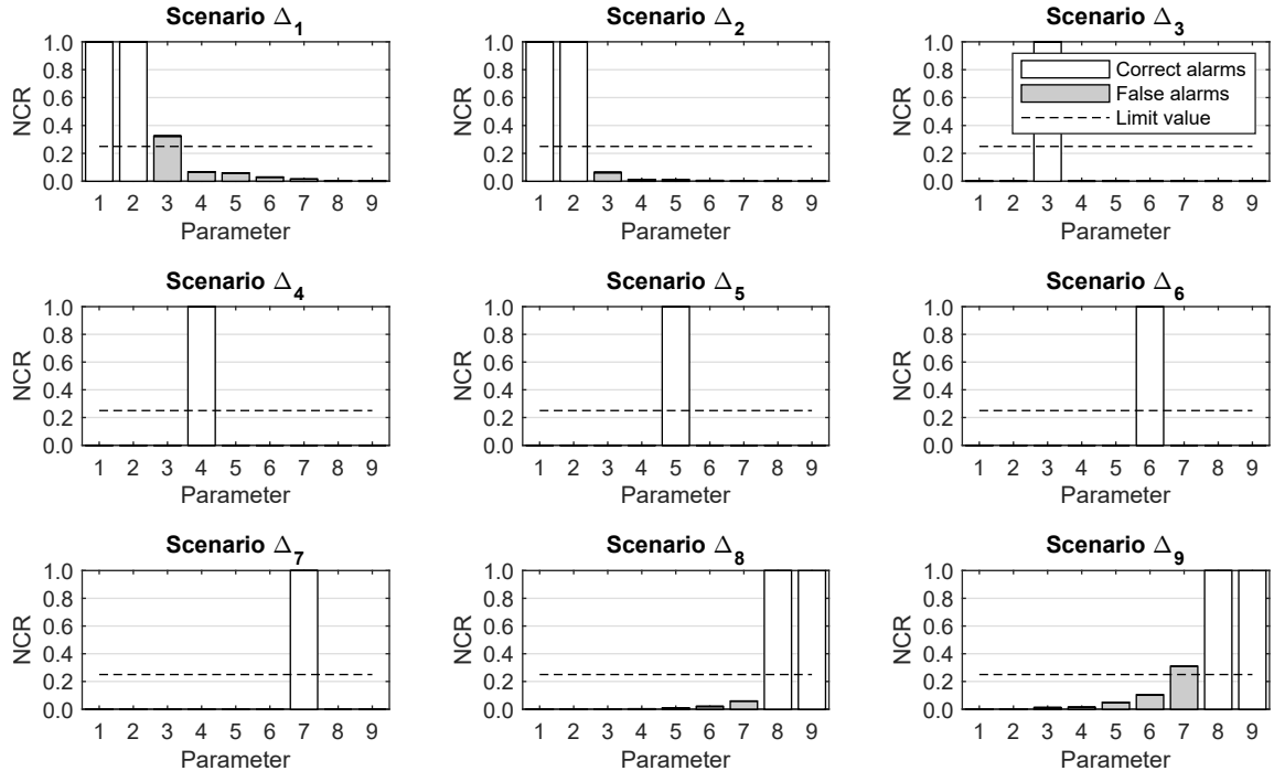
Figure 6: Non-centrality ratio for all nine damage scenarios
