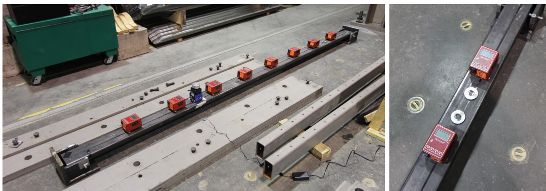
Figure 11: Photos of the laboratory experiment with a laboratory beam (left) and exemplary extra masses that increase the beam segment weight by 2.5% (right)
