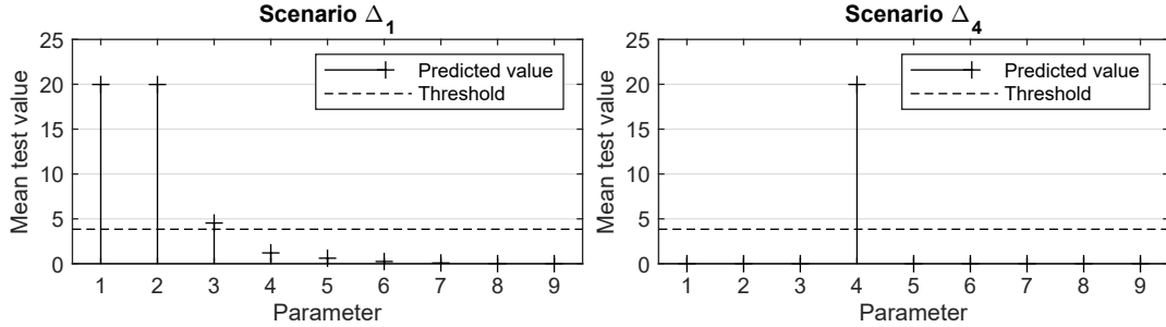
Figure 4: Predicted mean of the minmax localization test statistic for two damage scenarios and numerical data
