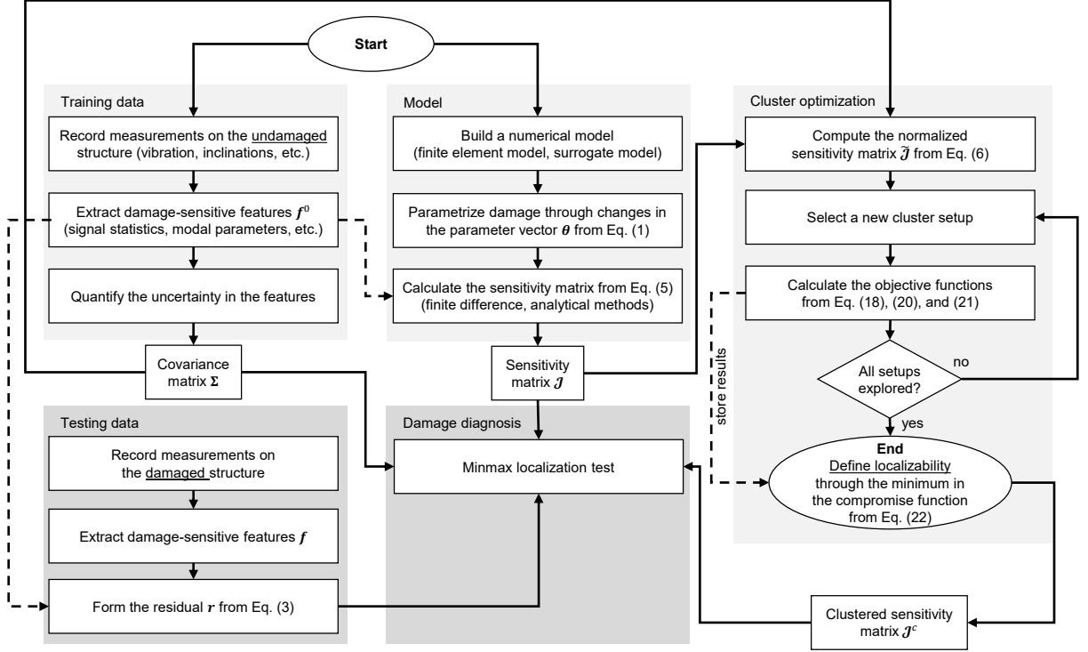
Figure 8: Flow chart of the optimization scheme, with the final result being the localizability assessment. Light grey boxes indicate that the analysis is based on data from the undamaged structure
