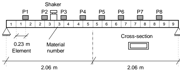
Figure 2: Finite element model in ANSYS
