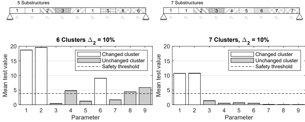
Figure 5: Mean of the minmax localization test statistic for six clusters (left) and seven clusters (right). Six clusters lead to a high detectability of damage in parameter 2, but seven clusters reduce false alarms
