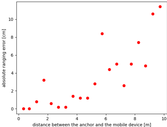
Fig. 6. Absolute ranging error between anchor and mobile device. Measurements are collected from the PWM output pin of the mobile device, while the ground truth is obtained by a laser distance meter.
